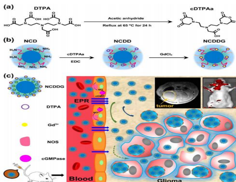
Figure 3. The creation of DTPA derivatives using acetic anhydride
