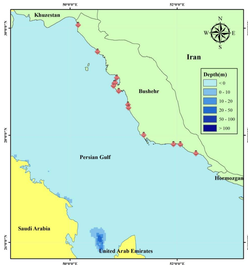
Figure 1: Map of the Persian Gulf showing fish landing sites along coasts (red dots).
