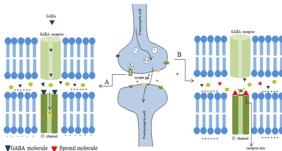
Figure 1: The mechanism of fipronil, A: normal state, B: the activity of fipronil on GABA chloride channels.
