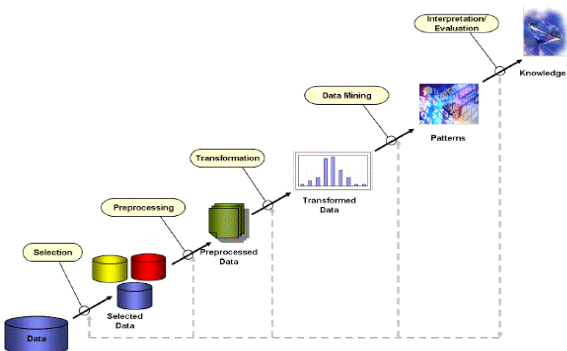
Fig 2 Steps of the KDD Process
