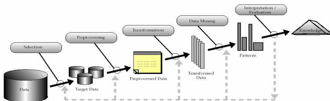
Figure 1 KDD process
