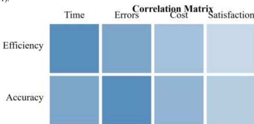
Figure 4: Correlation Matrix of Key Variables
