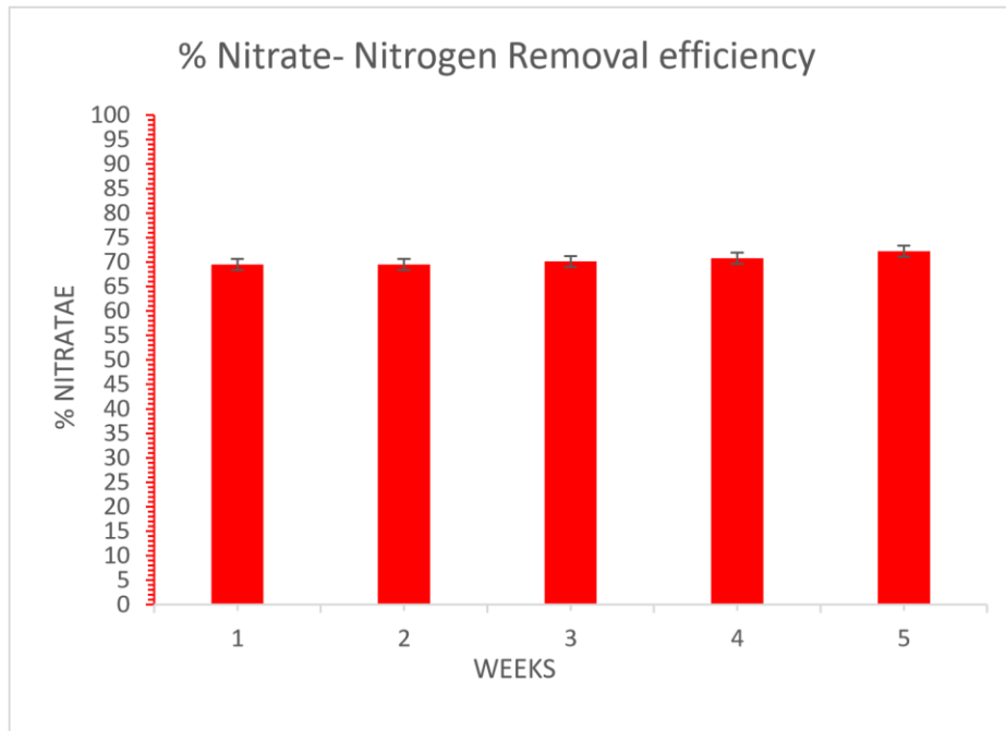
Fig 1: Percentage Nitrate- Nitrogen Removal efficiency
