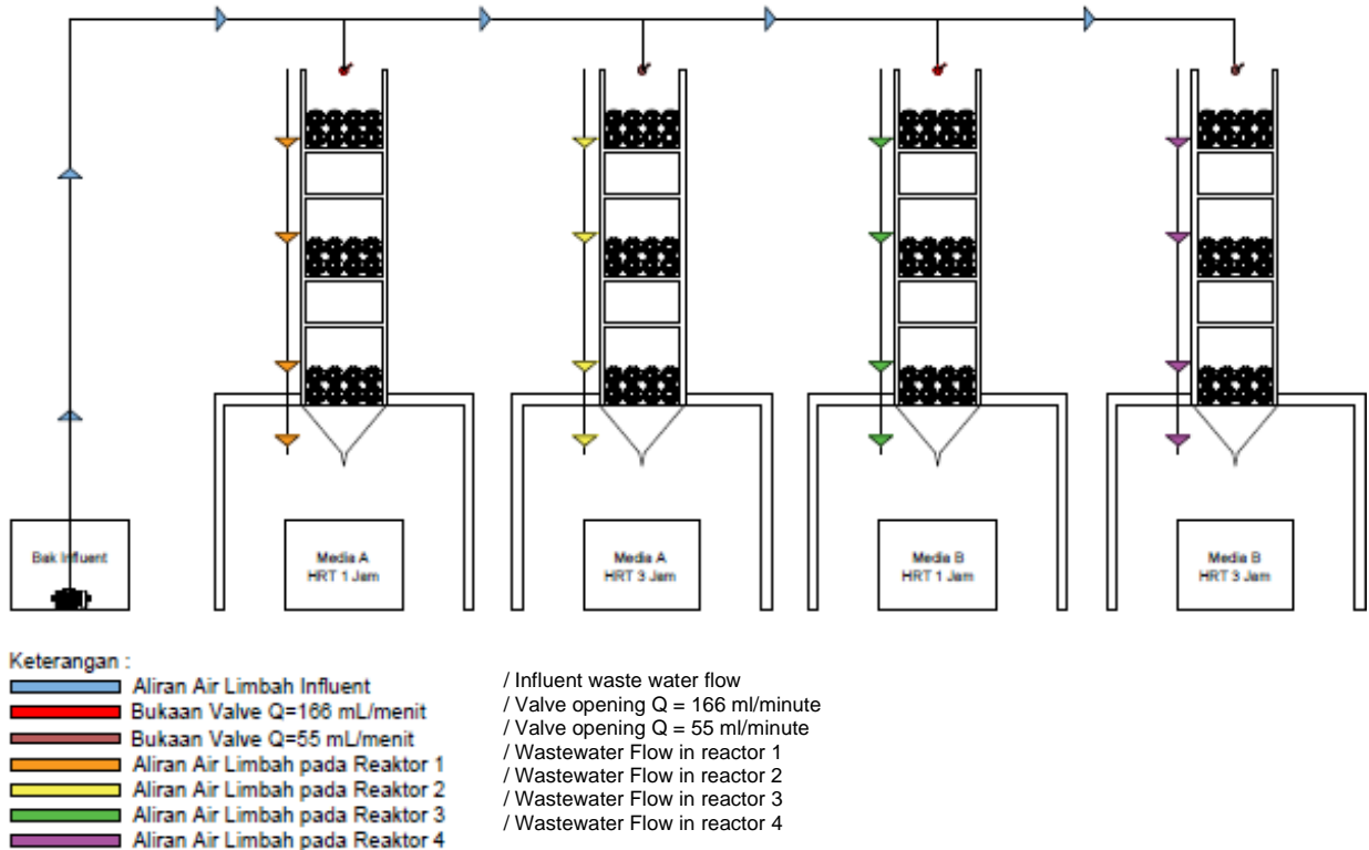
Figure 3 Reactor for running process
