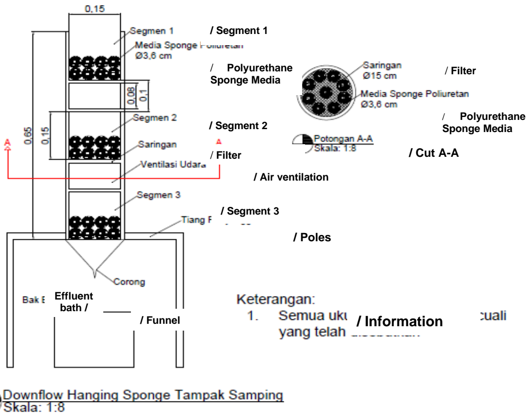
Figure 2 Design of downflow Hanging flow
