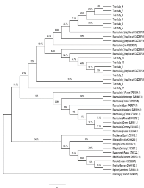
Figure 2. Shows Evolution tree for study samples and reference samples of R. auricularia snails in Basra province and the Republic of Iran.
